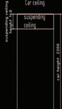
Car height
