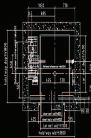
Hoistway top plane layout
