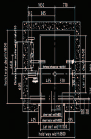
Hoistway plane layout
