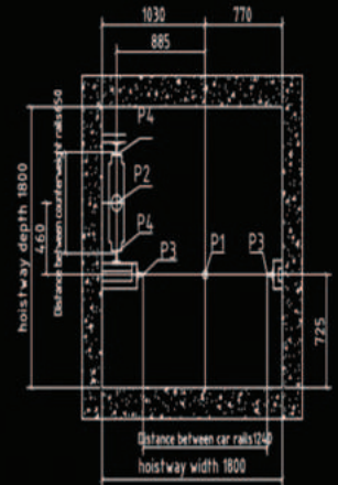
Pit plane layout
